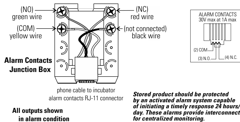
Figure 6-1. Contacts
