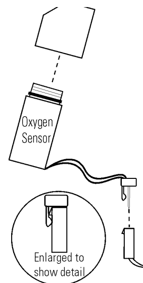
Figure 5-13. Detail
