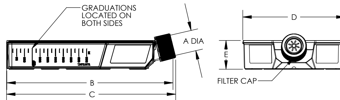
END VIEW
